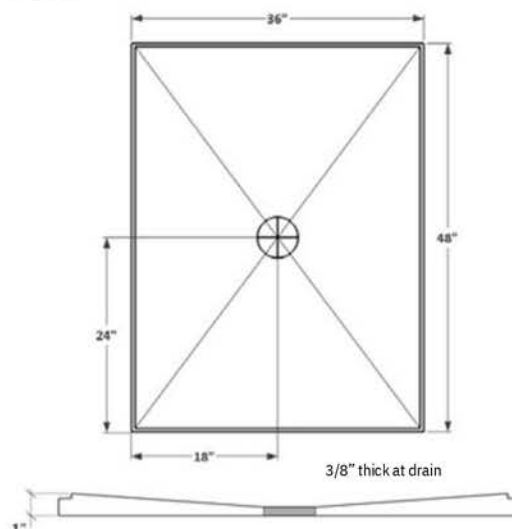
36" x 48" HBLPSP3648
