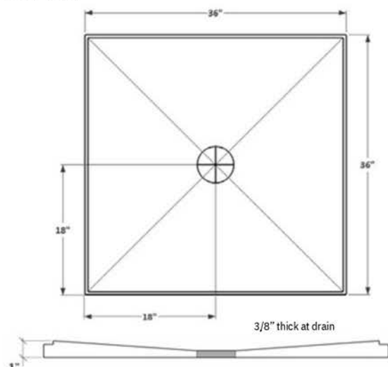
36" x 36" HBLPSP3636
