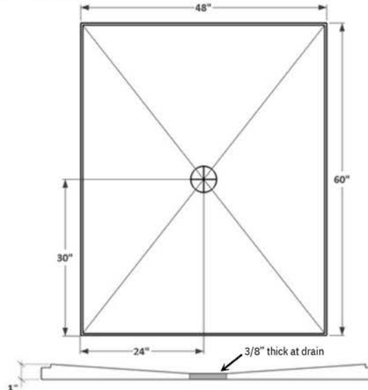
48" x 60" HBLPSP4860
