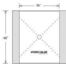
4' x 4' Shower Pan Cut to Size
