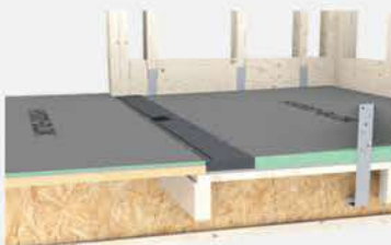
Single Slope Shower Pans
